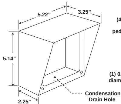
Front View of Optional VE-5x5 (not included)
