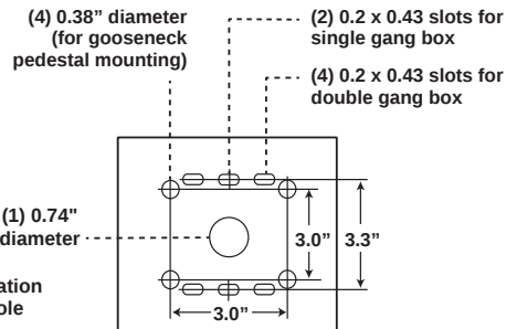
Rear View of VE-5x5 (not included)
