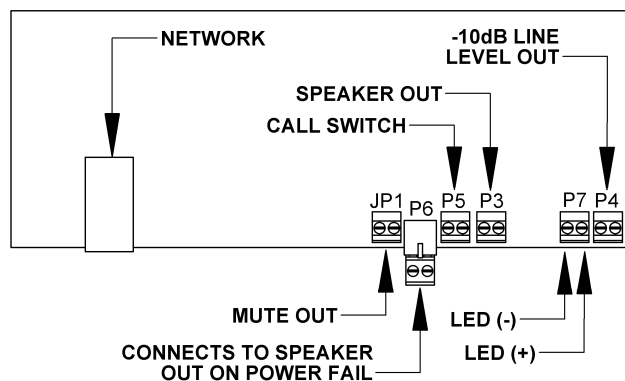
Figure 1. VIP-160 Connections
