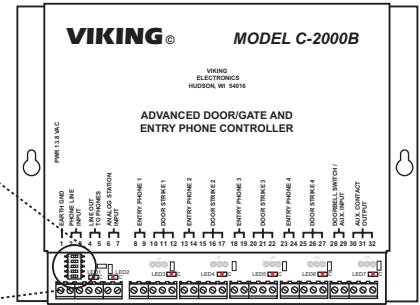
DIP Switches shown in the factory default positions
