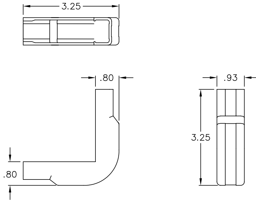
3/4" OUTSIDE CORNER COVER
