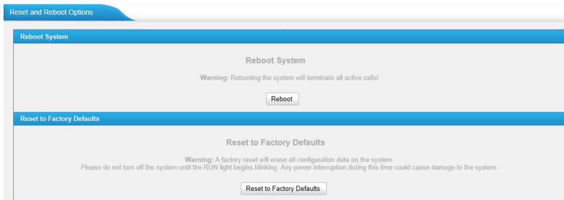
Figure 3-33 Reset and Reboot
